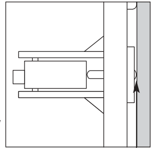
Tamper switch plunger must be pressed in fully by wall surface
